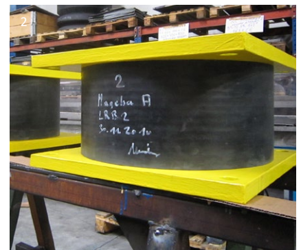
1 Testing of LASTO®LRB bearings 2 Manufacturing of LASTO®LRB bearings
