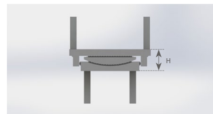
Section through KE bearing without anchor plates, with dowels
